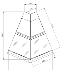
Vega S Corner OC 45
