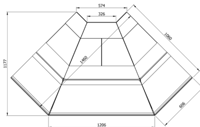
Vega S Corner OC 90
