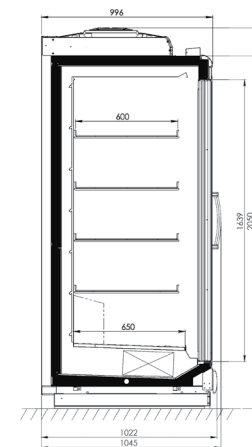
Erida plug-in L
