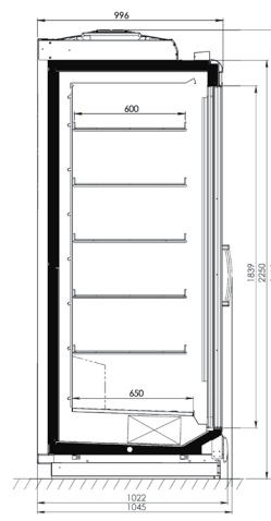
Erida plug-in H
